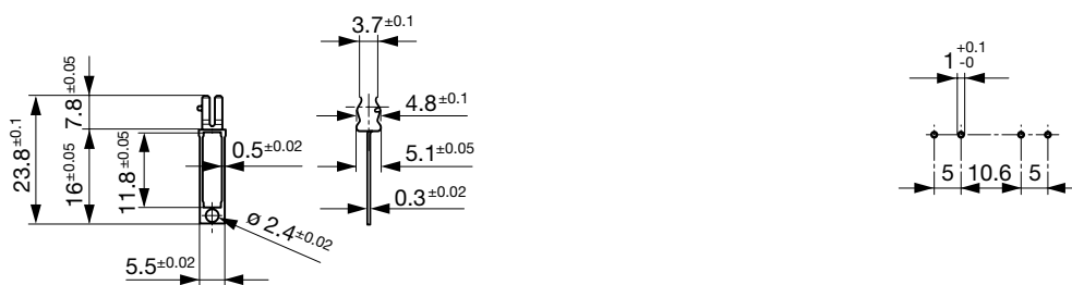
Drilling diagram
